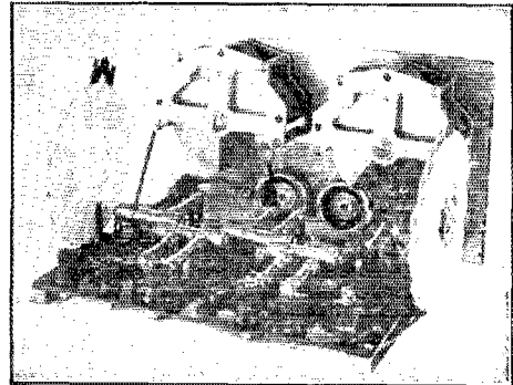
THE GARDINER & HEPBURN “RECTOFLEX” This set uses resistance-coupled audio, of which one stage is reflexed in the manner suggested by Fig. 1. The two coils are the inductances of the R. F. amplifier and are tuned by the variable condensers. The fat cartridges are the coupling capacities, while the slender ones are the grid leaks and plate resistances.
