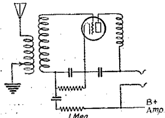
FIG. 1 SHOWING ONLY THE REFLEXED TUBE
